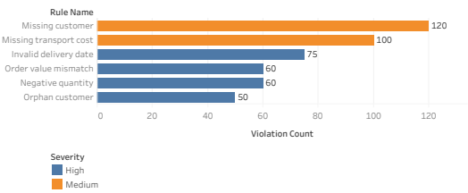
Data Quality Issues by Rule
